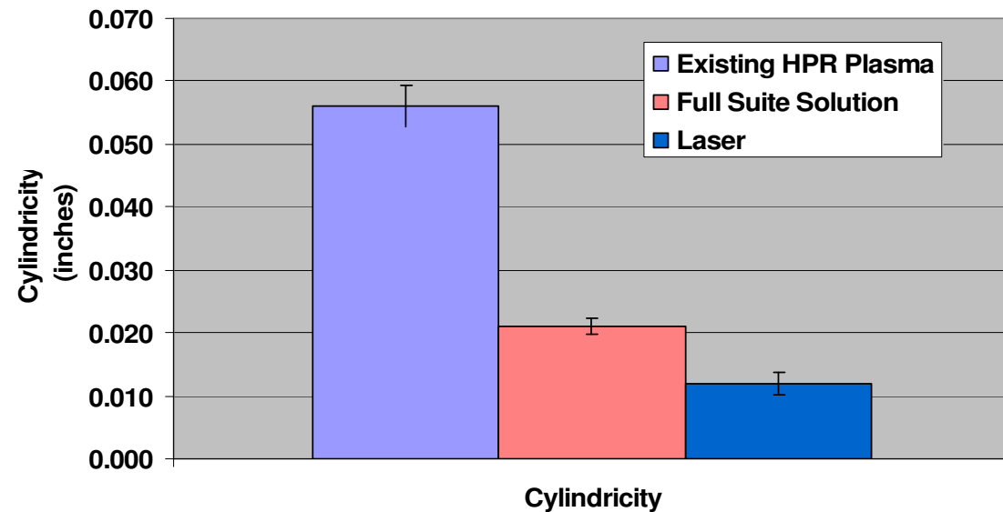
12 mm (1/2") hole with True Hole technology
