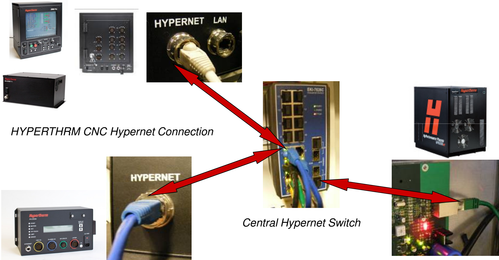
HPRXD Hypernet Communication (replaces serial connection)
